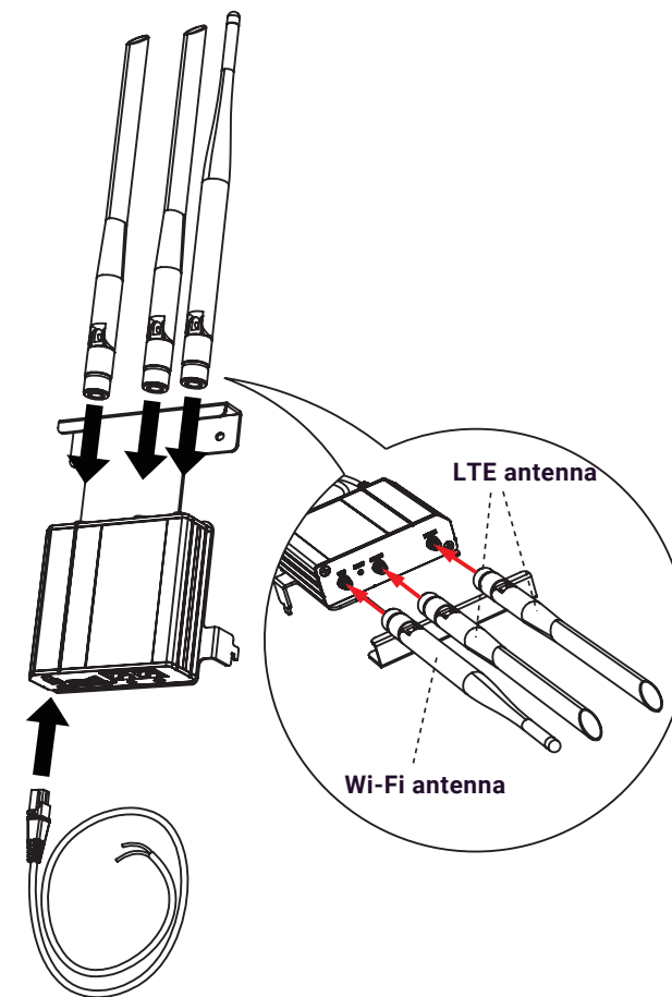
Step 4. Install power cable and 3 antennas on RUT240 router
