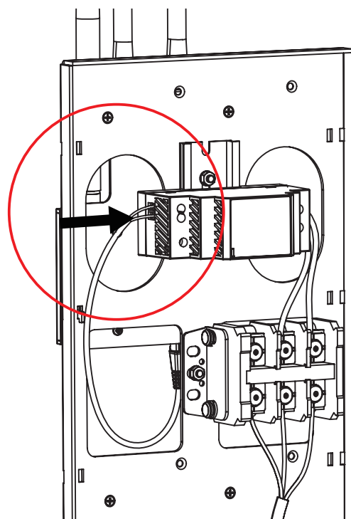
Step 6. Connect power cable from RUT240 router
